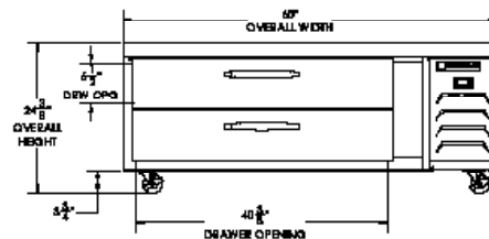
ELEVATION VIEW
